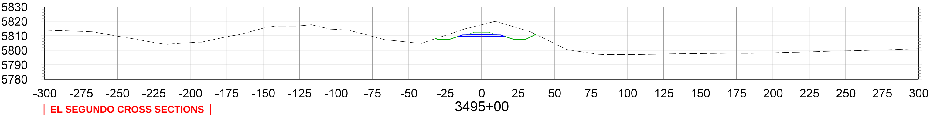
CROSS SECTIONS STA.3495+00 TO STA.3510+00
