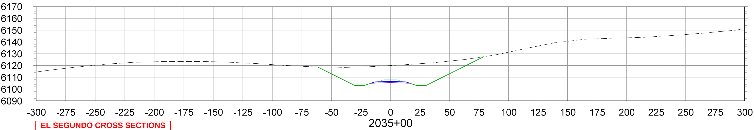
CROSS SECTIONS STA.2035+00 TO STA.2050+00
