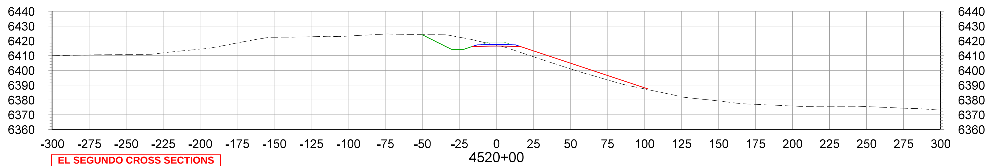
CROSS SECTIONS STA.4520+00 TO STA.4530+00
