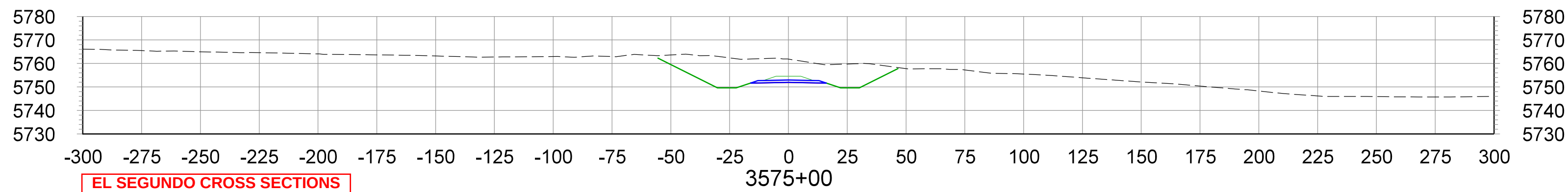
CROSS SECTIONS STA.3575+00 TO STA.3590+00
