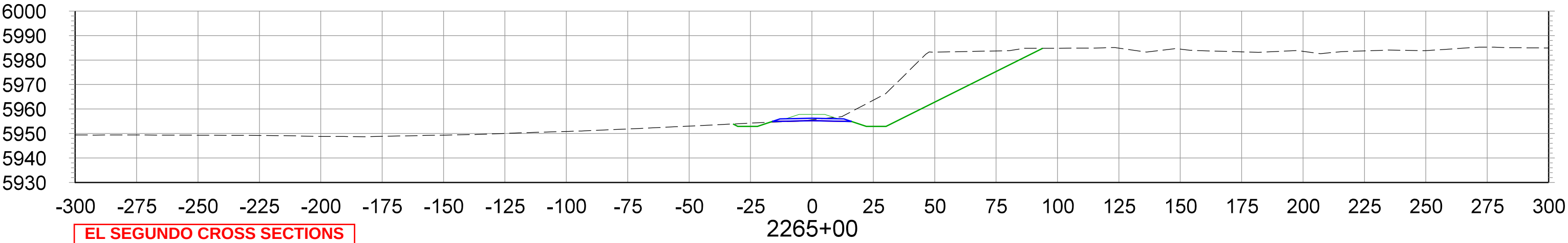
CROSS SECTIONS STA.2265+00 TO STA.2280+00
