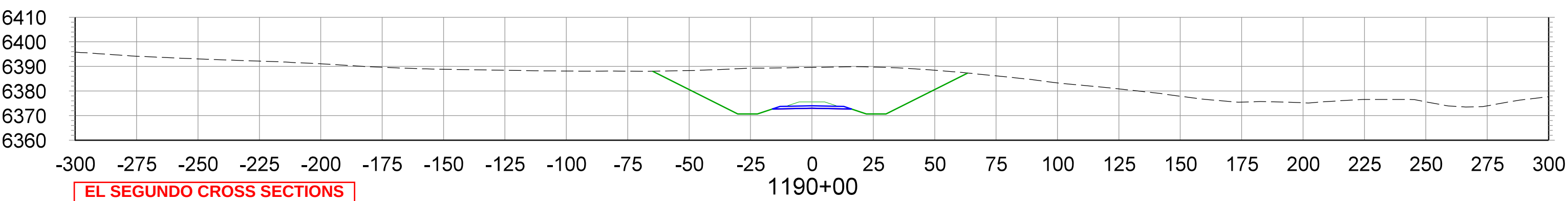
CROSS SECTIONS STA.1190+00 TO STA.1205+00
