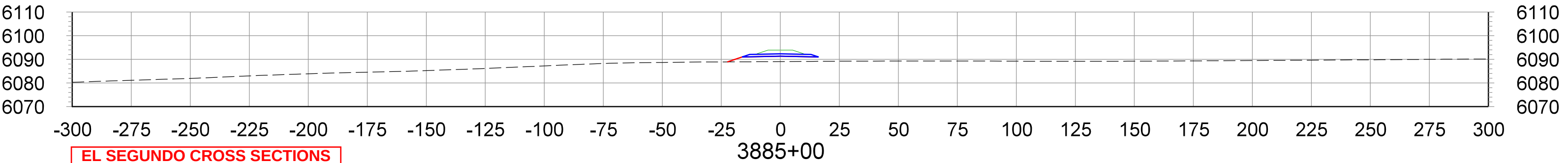
CROSS SECTIONS STA.3885+00 TO STA.3900+00
