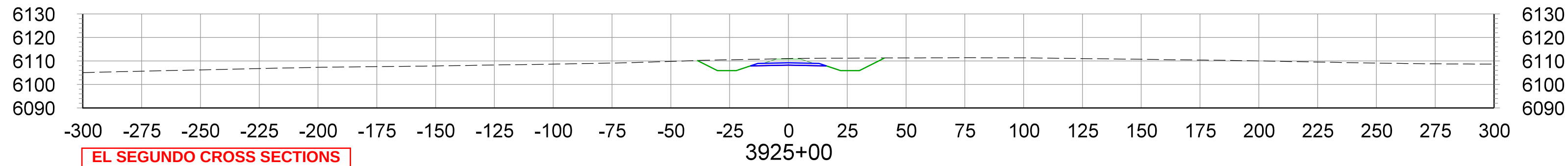
CROSS SECTIONS STA.3925+00 TO STA.3940+00
