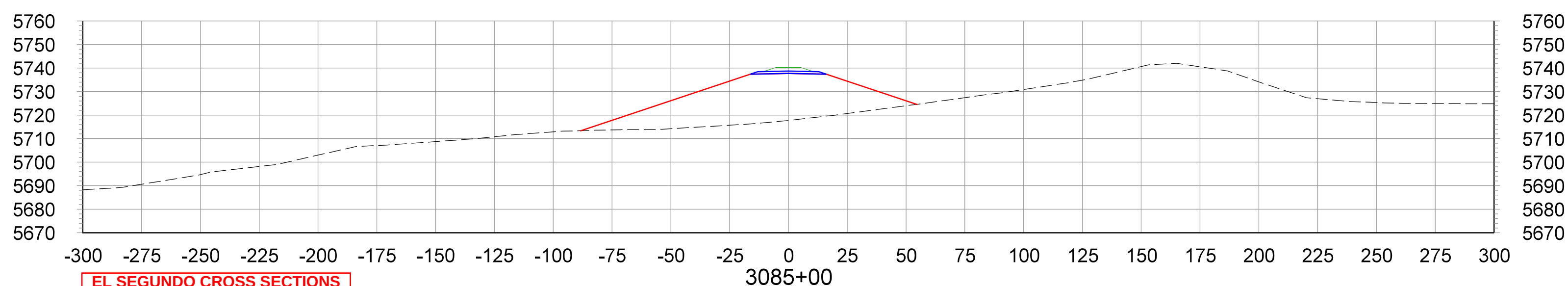
CROSS SECTIONS STA.3085+00 TO STA.3095+00
