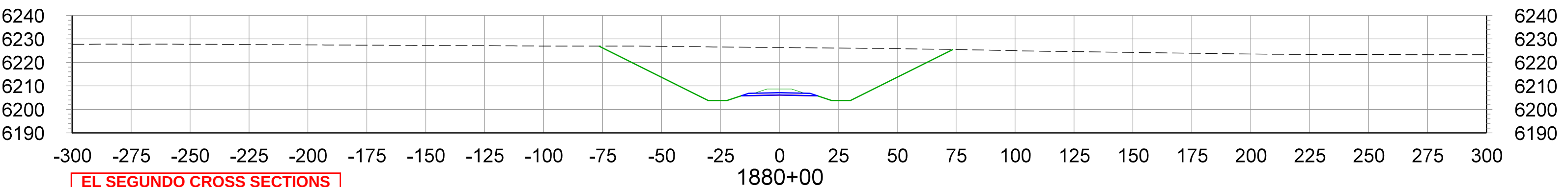
CROSS SECTIONS STA.1880+00 TO STA.1895+00
