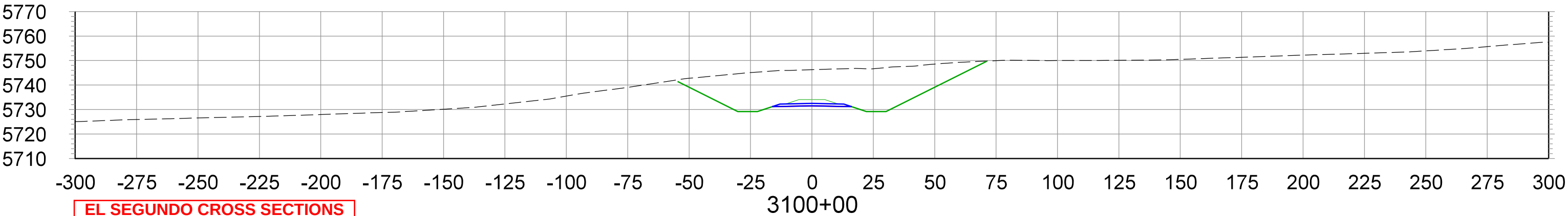
CROSS SECTIONS STA.3100+00 TO STA.3115+00
