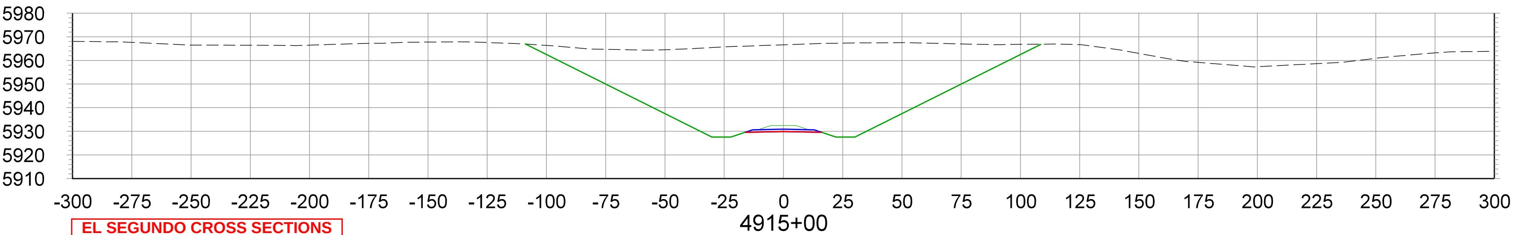
CROSS SECTIONS STA.4915+00 TO STA.4930+00
