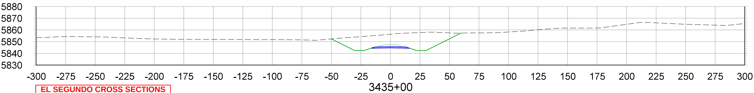
CROSS SECTIONS STA.3435+00 TO STA.3450+00
