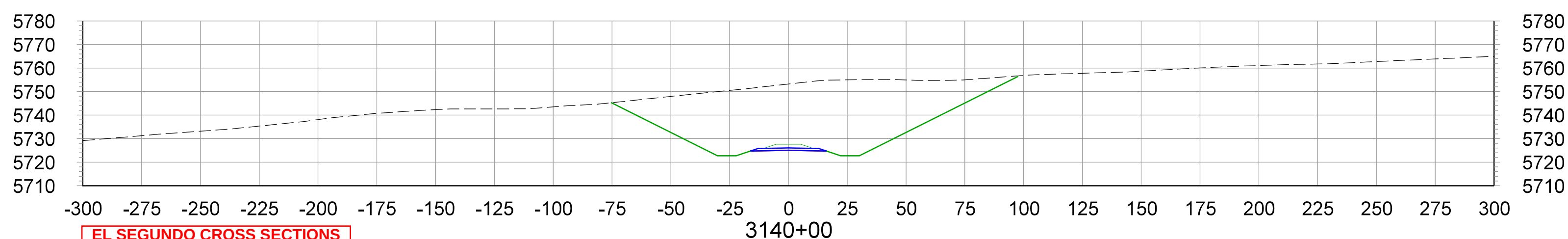
CROSS SECTIONS STA.3140+00 TO STA.3150+00
