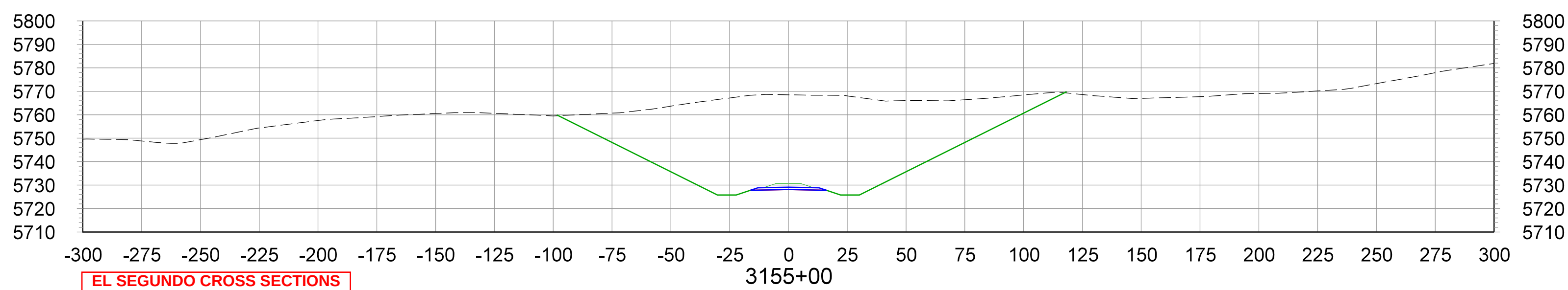
CROSS SECTIONS STA.3155+00 TO STA.3165+00
