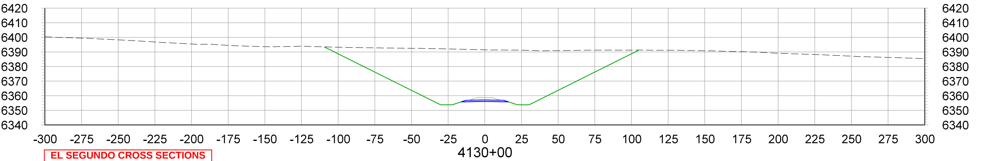
CROSS SECTIONS STA.4130+00 TO STA.4145+00
