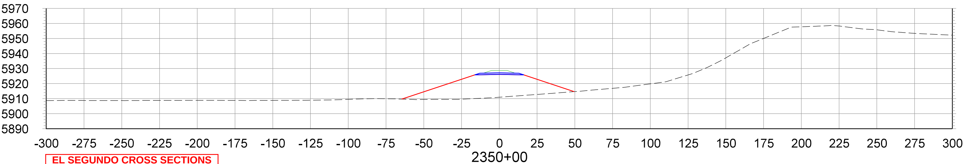
CROSS SECTIONS STA.2350+00 TO STA.2360+00
