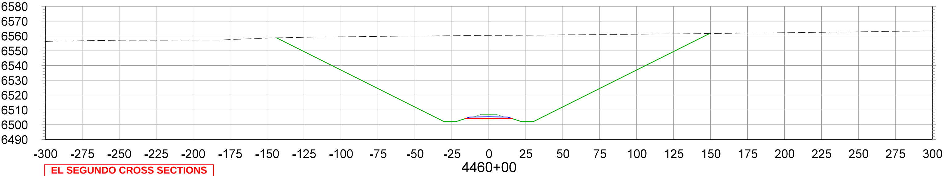
CROSS SECTIONS STA.4460+00 TO STA.4470+00
