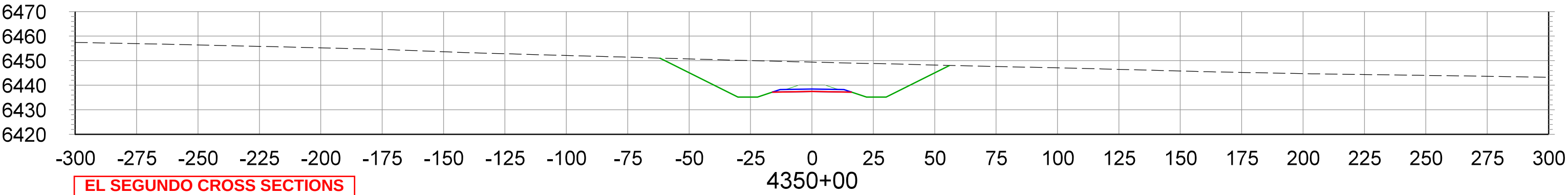
CROSS SECTIONS STA.4350+00 TO STA.4365+00
