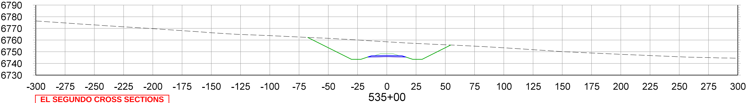
CROSS SECTIONS STA.535+00 TO STA.550+00
