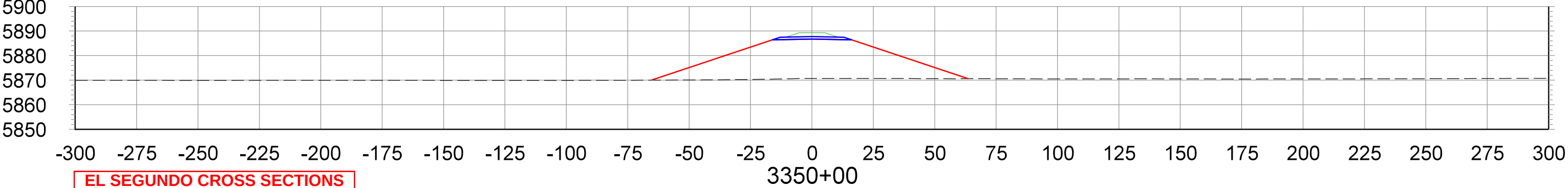
CROSS SECTIONS STA.3350+00 TO STA.3370+00
